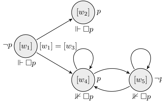
Figura fil.3: The filtration of the model in Figura fil.2 .
