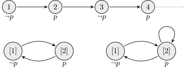
Figura fil.1: An infinite model and its filtrations.
