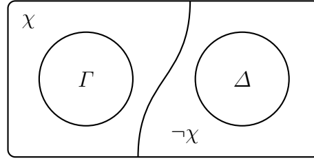
Figura 3.1: \chi separates \Gamma and \Delta
