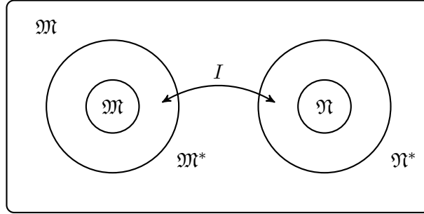
Figura 4.1: The estrutura \mathfrak{M} with the internal partial isomorphism.
