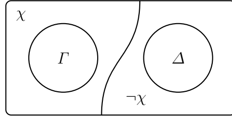
Figura int.1: \chi separates \Gamma and \Delta
