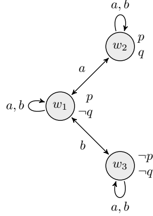
Figura 1: A simple epistemic model.
